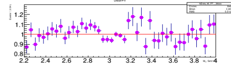
for 'FS' J/ψ Candidates
