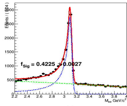
for 'FS' J/ψ Candidates
