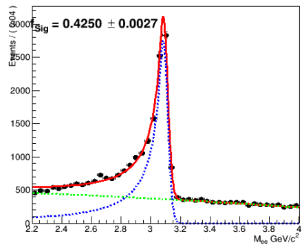
for 'FS' J/ψ Candidates
