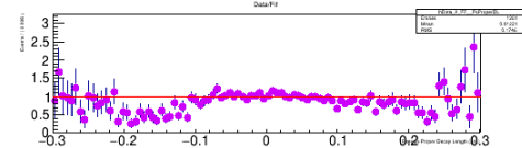
A RooPlot of "Pseudo-Proper Decay Length (cm.)"
