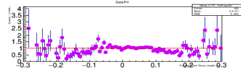
A RooPlot of "Pseudo-Proper Decay Length (cm.)"
