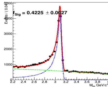
for 'FF' J/ψ Candidates
