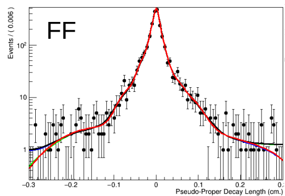
A RooPlot of "Pseudo-Proper Decay Length (cm.)"
