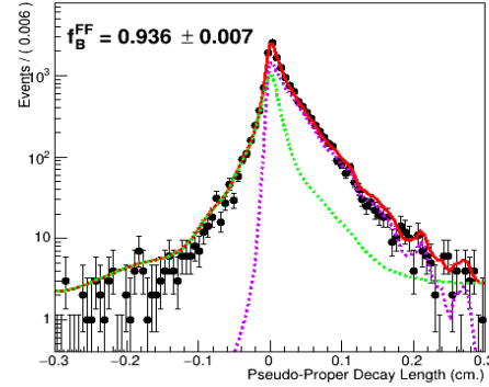
A RooPlot of "Pseudo-Proper Decay Length (cm.)"
