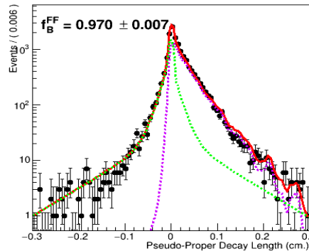
A RooPlot of "Pseudo-Proper Decay Length (cm.)"
