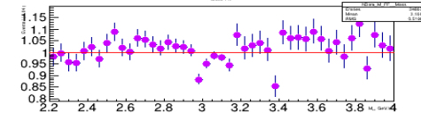
for 'FS' J/ψ Candidates
