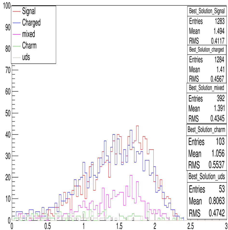
p_ltag after all cuts
