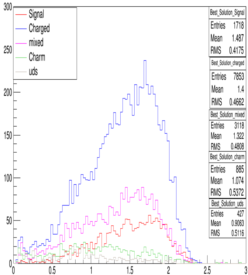
p_ltag after only abs(m_D-1.865)<0.03 cut
