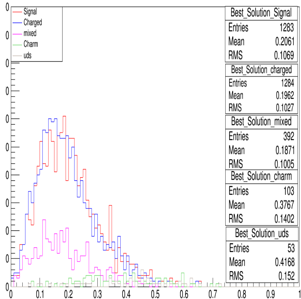
foxWolframR2 with all cuts
