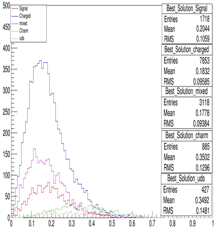
foxWolframR2 with only \text{abs}(m_D - 1.865) < 0.03 cuts
