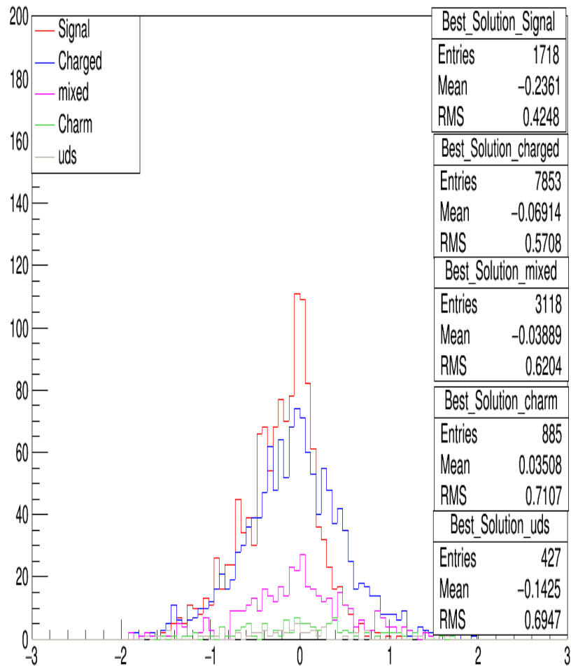
best cos_1+cos_tag with only abs(m_D-1.865)<0.03 cut
