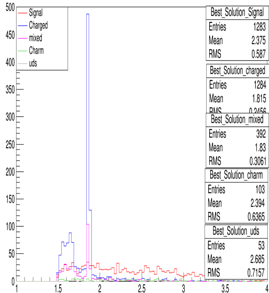
m_Kpi with all cuts
