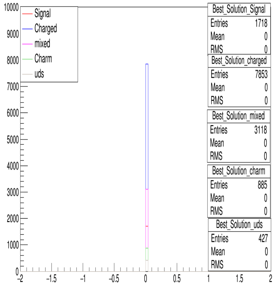
nK_L_sig with only \text{abs}(m_D - 1.865) < 0.03 cuts
