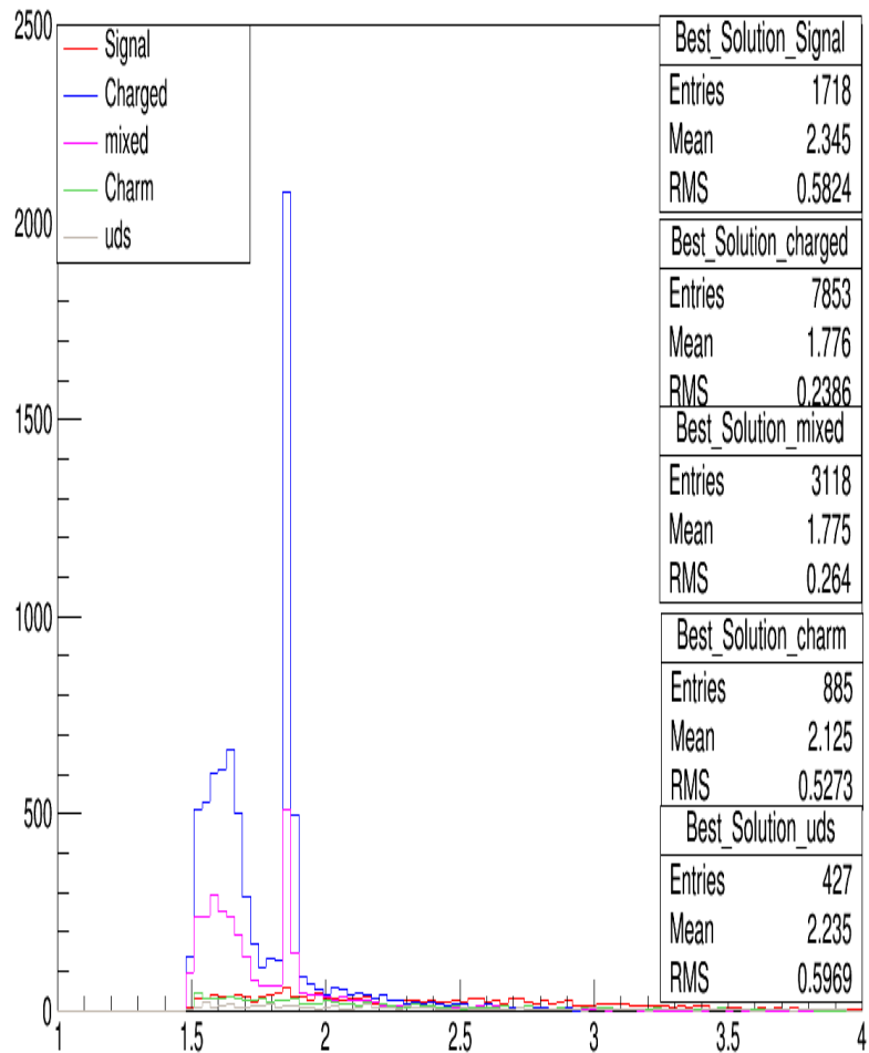
m_Kpi with only abs(m_D-1.865)<0.03 cut
