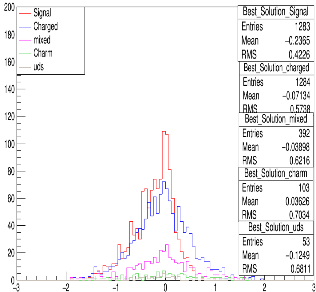
best cos_1+cos_tag with all cuts
