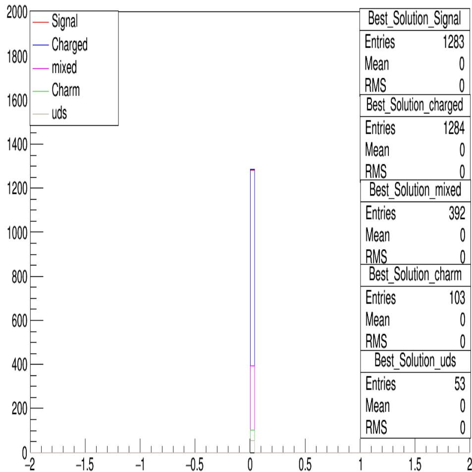
nK_L_sig with all cuts
