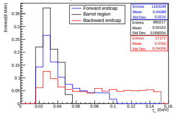
goodBelleGamma==0
