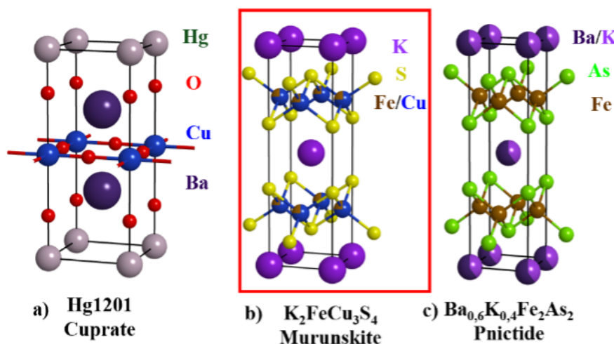
Figure 1: Comparison of murunskite structure b) with a cuprate a) and pnictide c)
