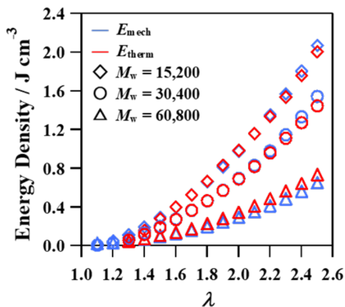
Figure 1: E_{mech} and E_{therm} of polyurethane rubbers with different crosslinking densities at different stretching ratios ( \lambda = l/l_0 ) from 1.0 to 2.6. M_w s represent the averaged molecular weights between the two crosslinks.
